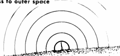
Long waves mostly absorbed or pass to outer space
